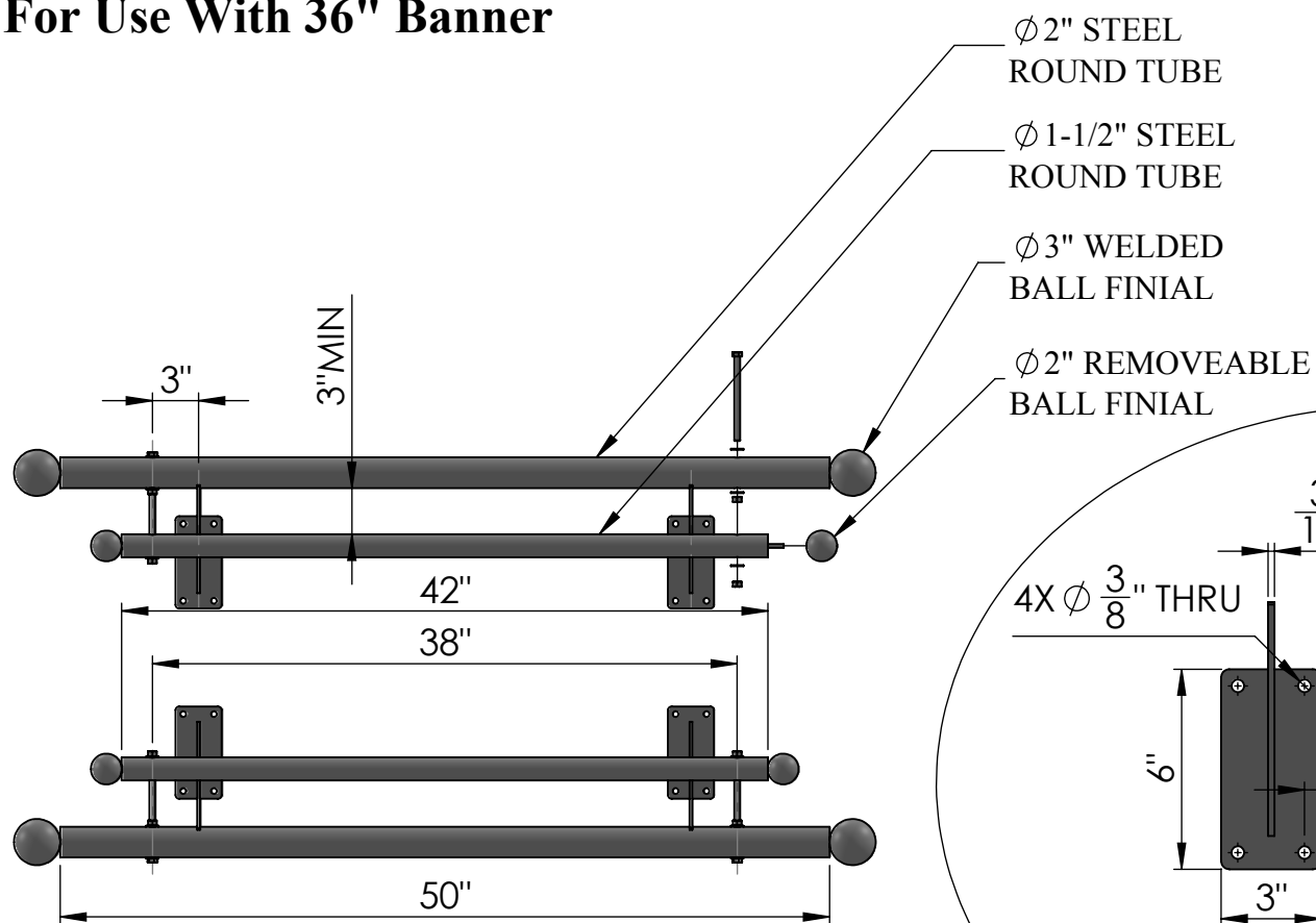
FRONT VIEW
