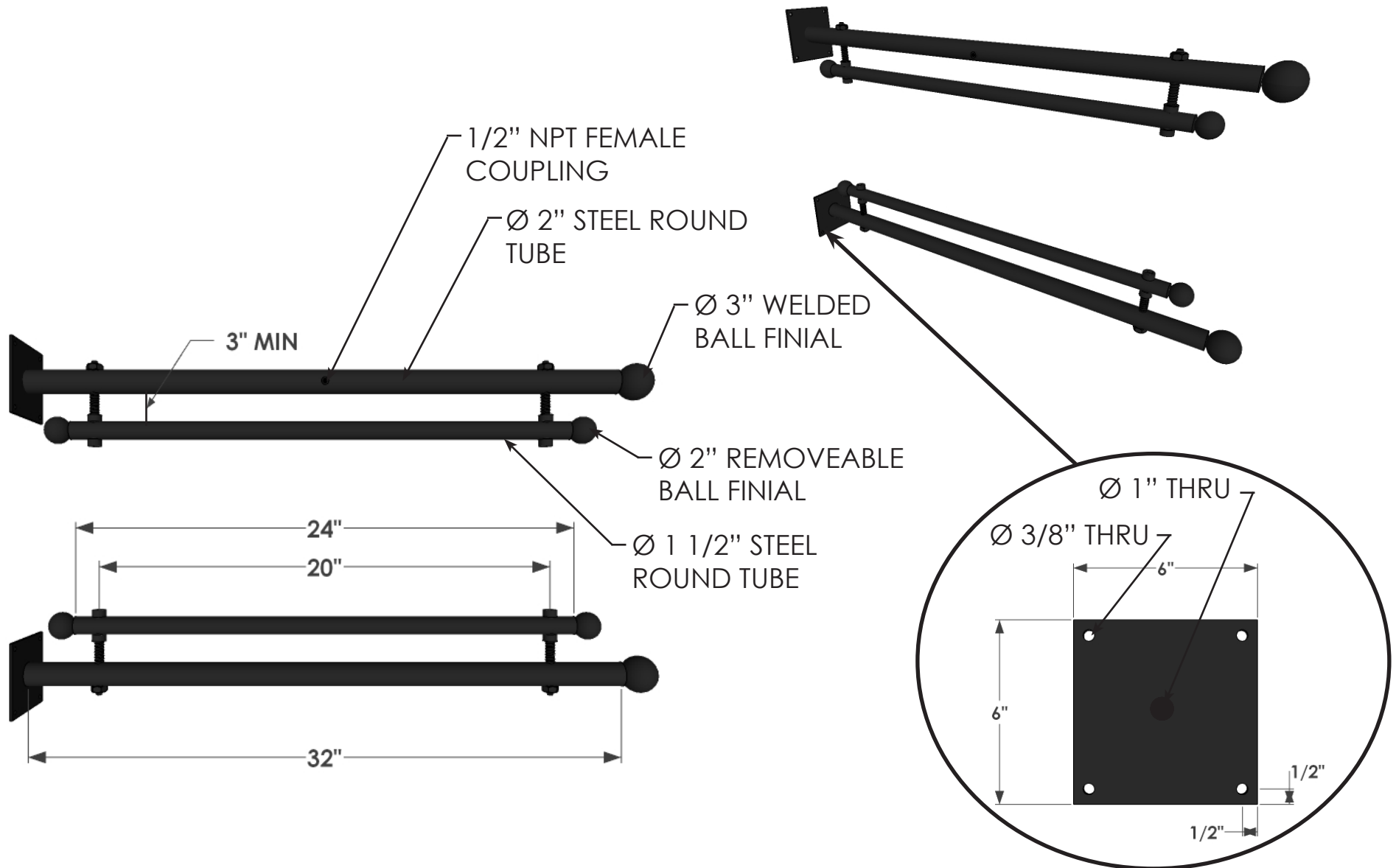
MOUNTING PLATE DETAIL
