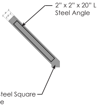
DETAIL VIEW
