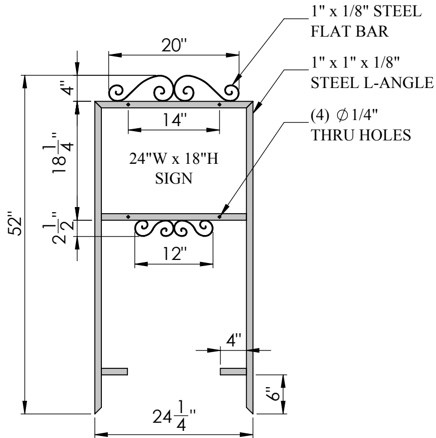
FRONT VIEW
