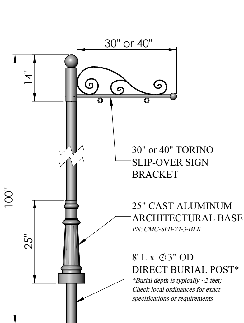
FRONT VIEW
