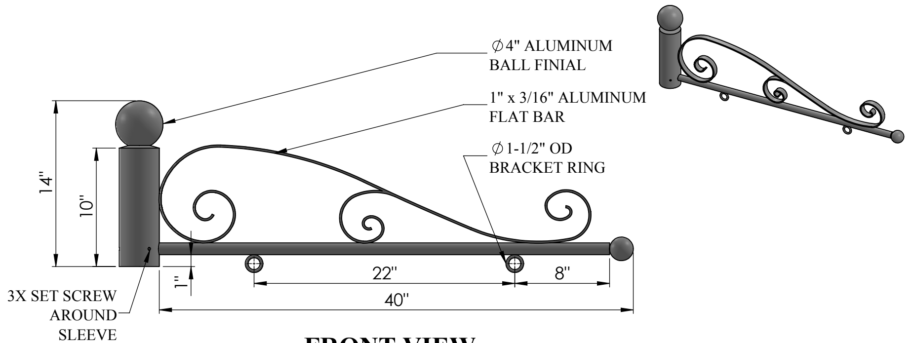
FRONT VIEW
