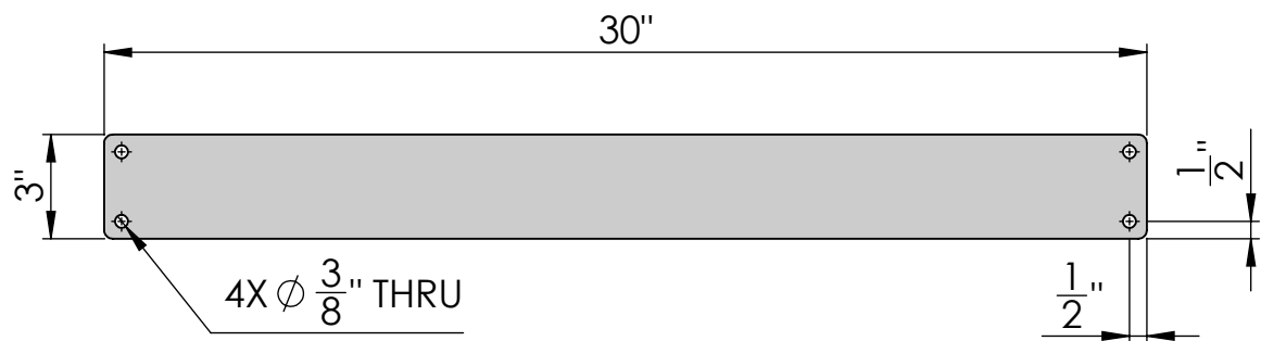
TOP VIEW
