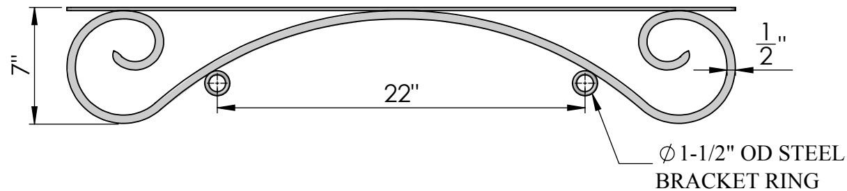
FRONT VIEW
