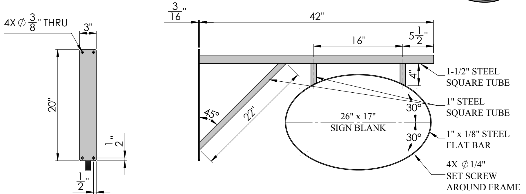
SIDE VIEW
