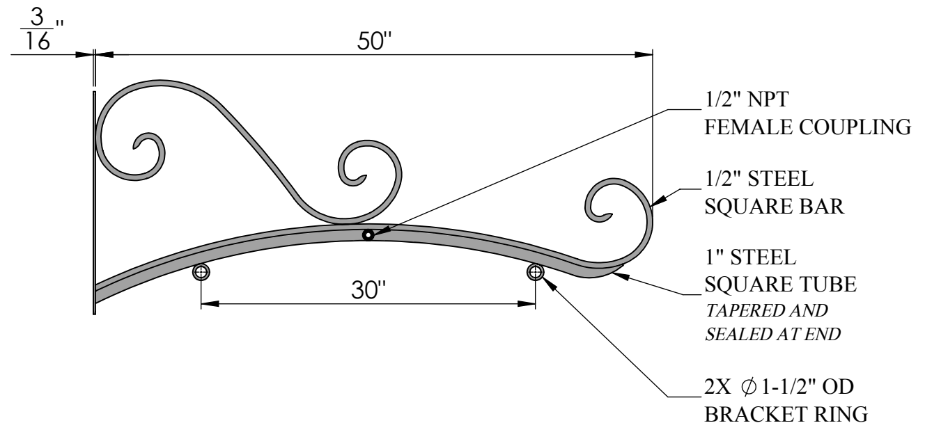
FRONT VIEW
