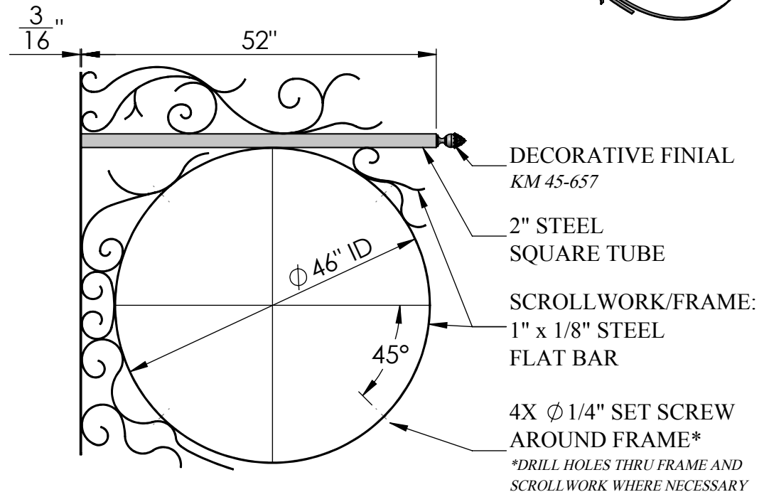
FRONT VIEW
