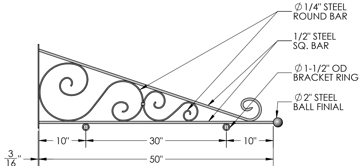
FRONT VIEW
