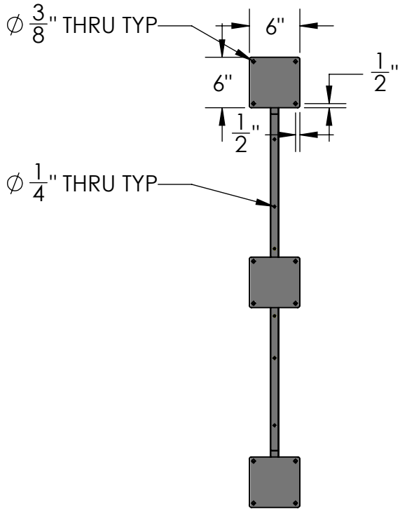
SIDE VIEW
