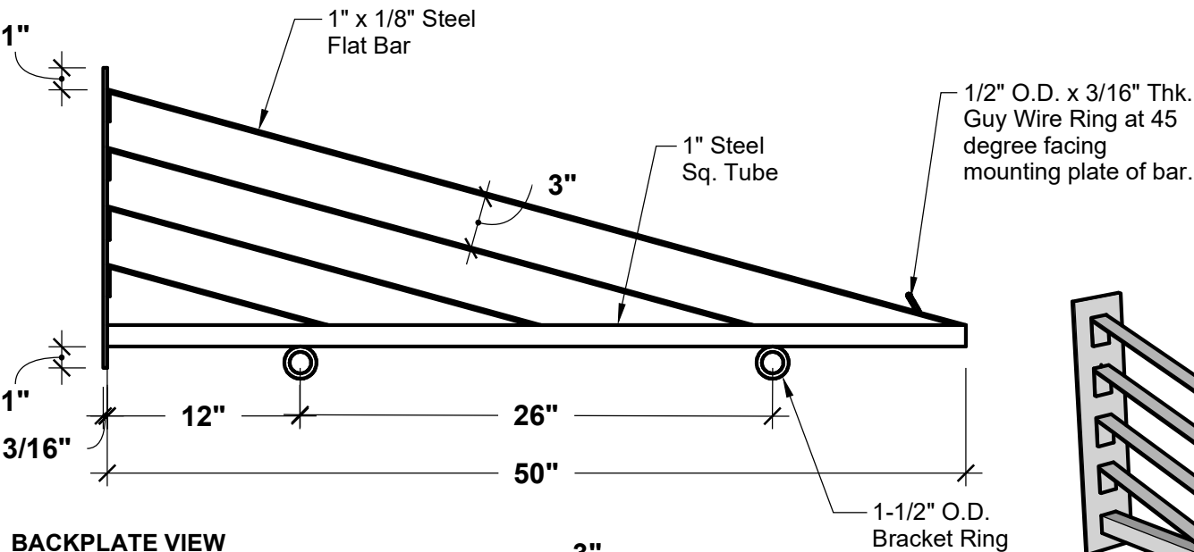
BACKPLATE VIEW
