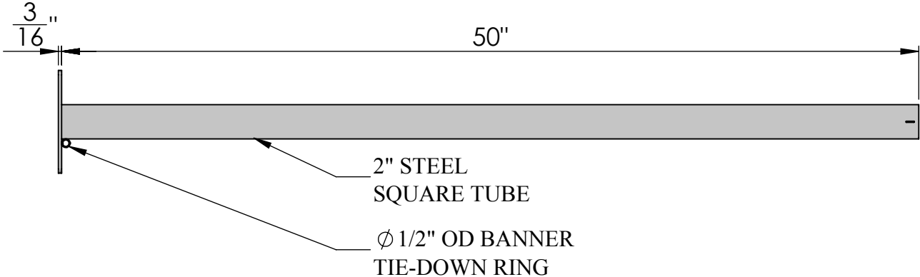
FRONT VIEW
