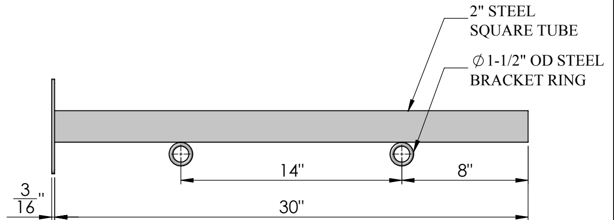
FRONT VIEW
