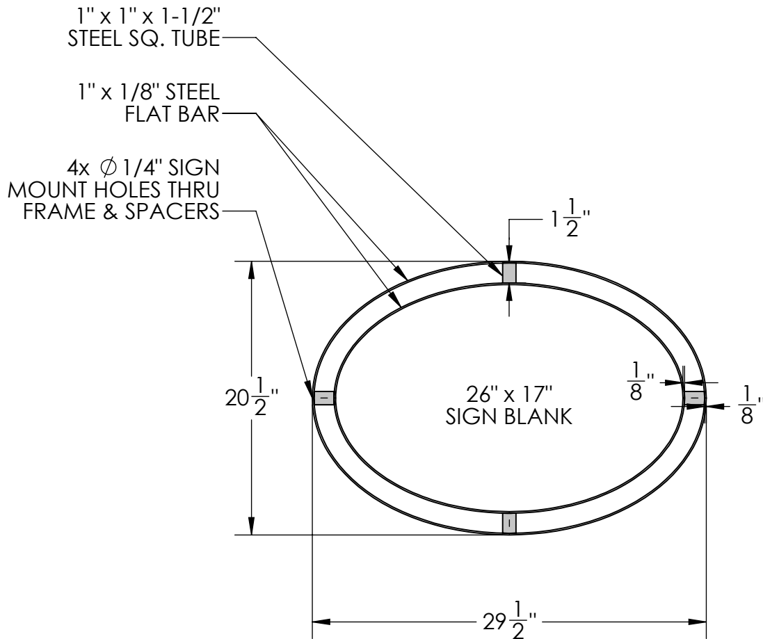
FRONT VIEW
