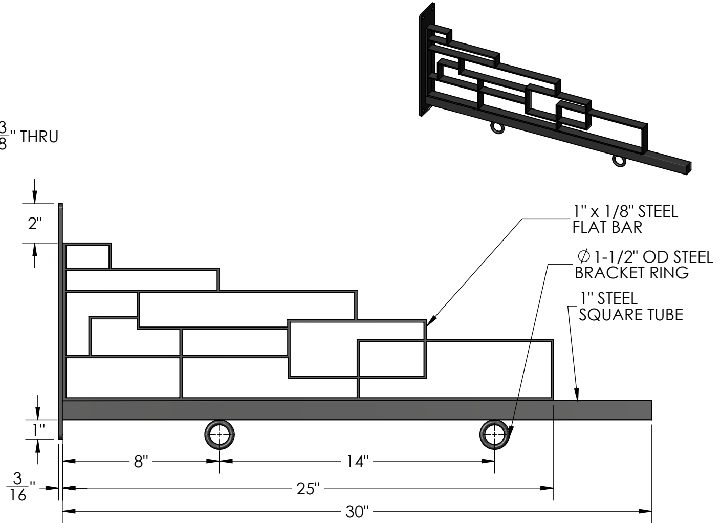
FRONT VIEW
