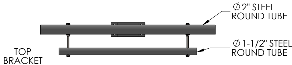
SECTION B-B
