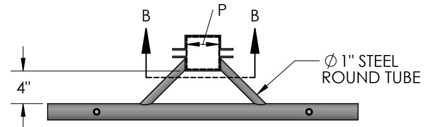
TOP VIEW
