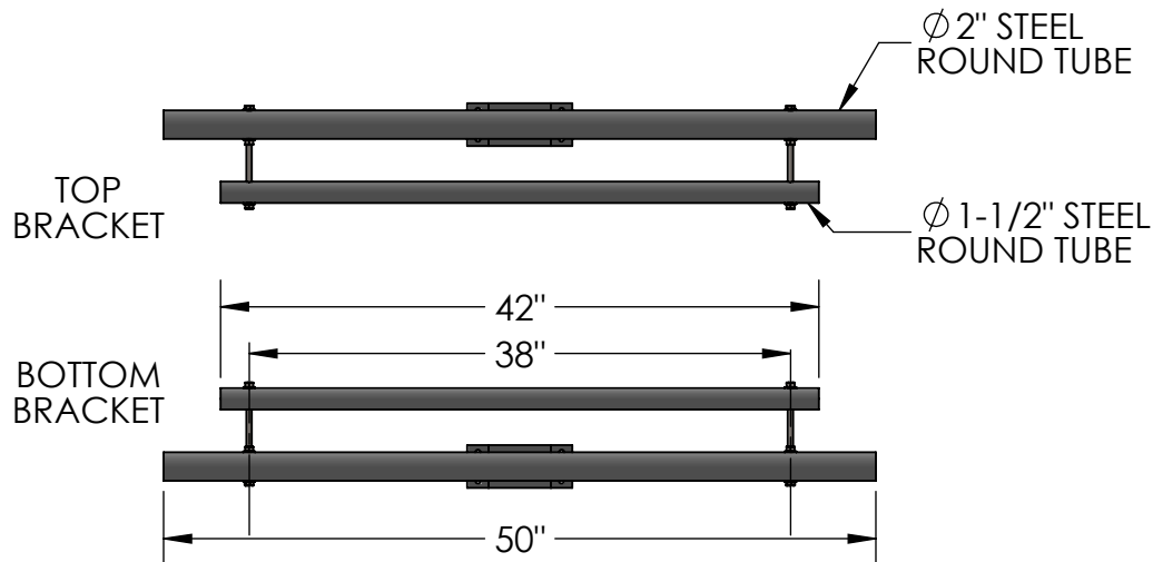
FRONT VIEW
