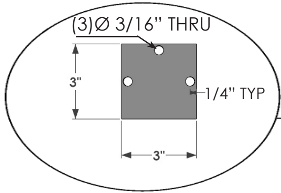
GUY WIRE PLATE DETAIL
