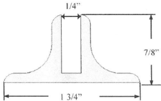
1/4" CHANNEL
