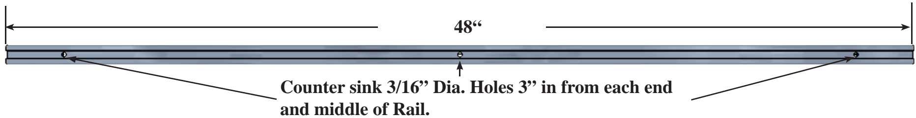
RAIL PROFILE
